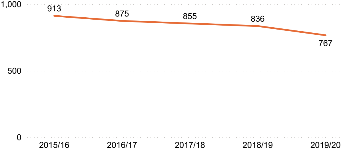
Total CO 2 emissions for North Tyneside (kilotons CO 2 )
